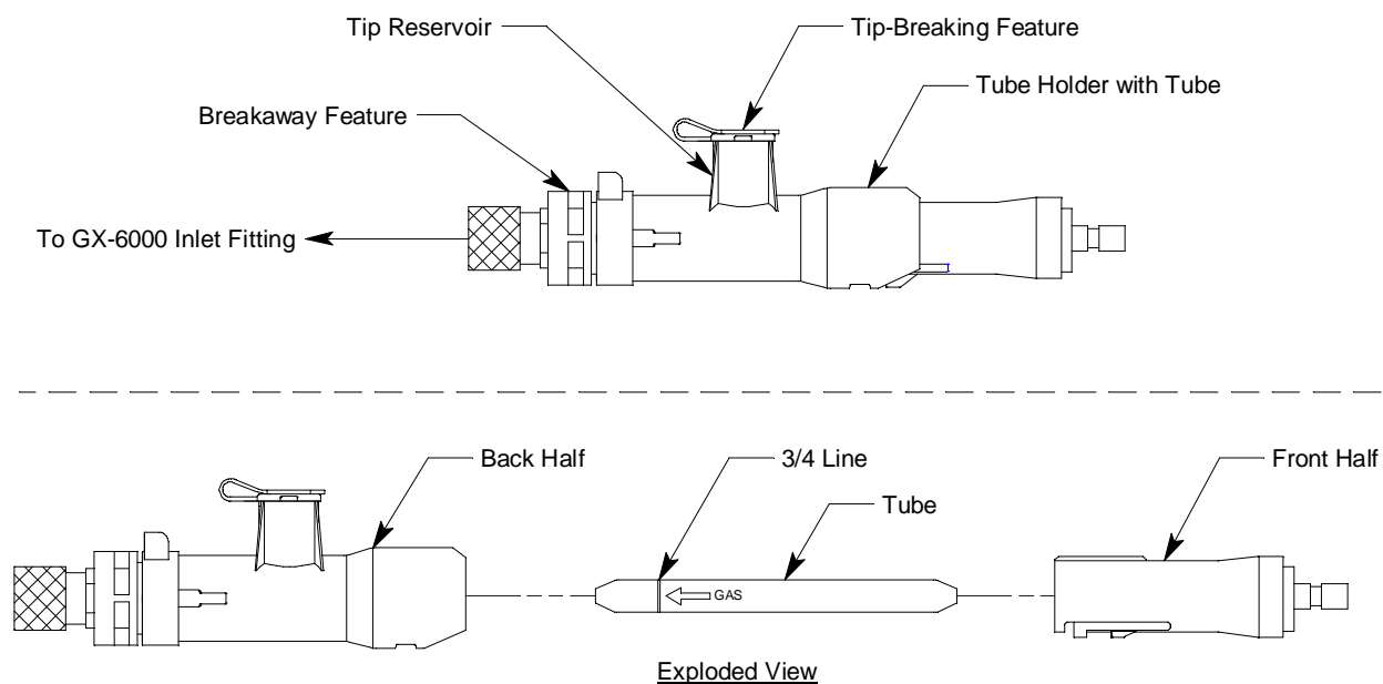
Figure 32: Tube Holder Component Location
