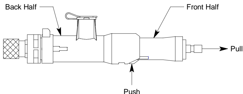
Figure 33: Replacing a Tube
